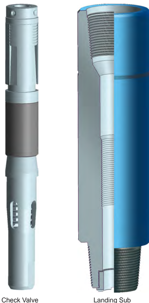
FT Type Drop-in Check Valve (F03)
