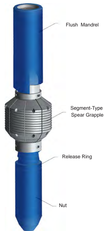
Spear Assembly with Flush Type Mandrel
