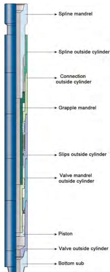
JYSZ Double Acting Hydraulic-Mechanical Drilling Jar (17)
