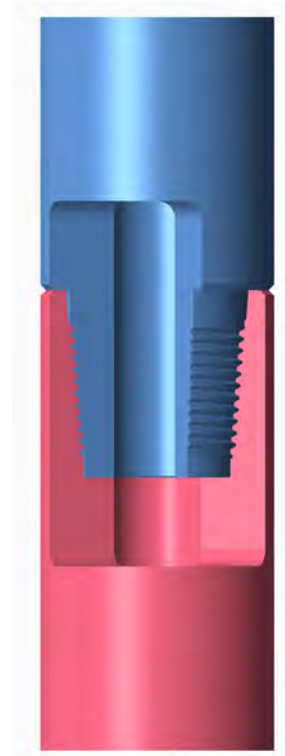
THDS Threaded Connection
